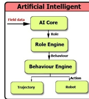
Fig. 8. Artificial Intelligence Algorithm
